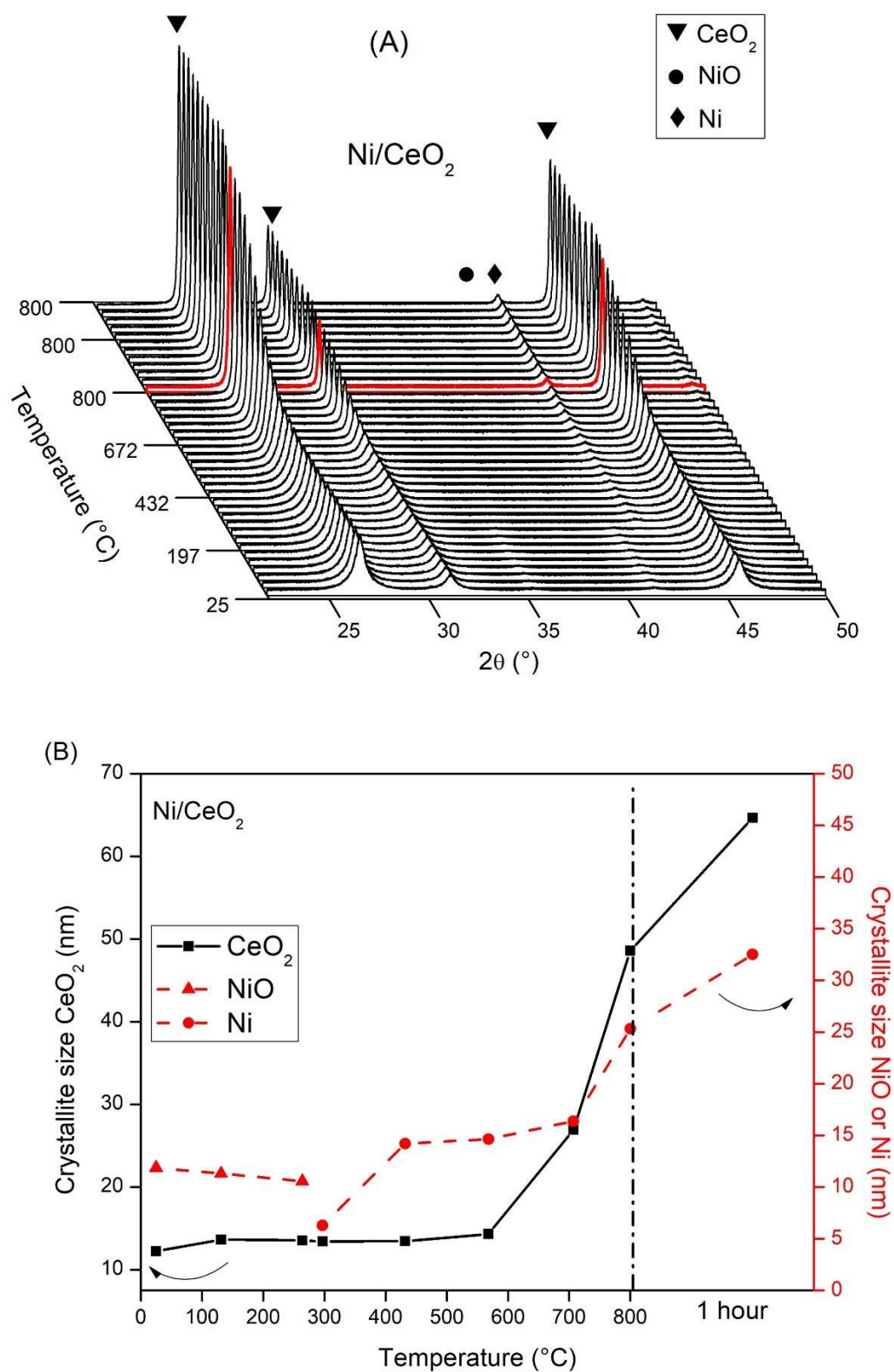
Figure 4.10. (A) X-ray diffraction patterns obtained during reduction from room temperature to 800 °C for Ni/CeO 2 ; (B) Crystallite size of NiO, Ni 0 and CeO 2 during the reduction process.
