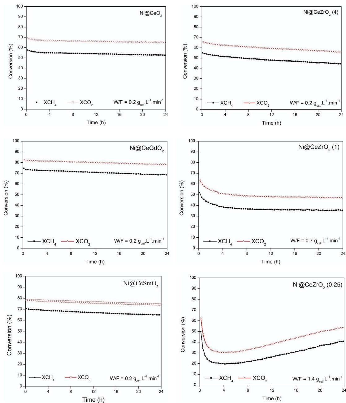
Figure 5.6. Conversion of \text{CH}_4 and \text{CO}_2 during DRM at 800 °C and \text{CH}_4/\text{CO}_2 molar ratio of 1.0.
