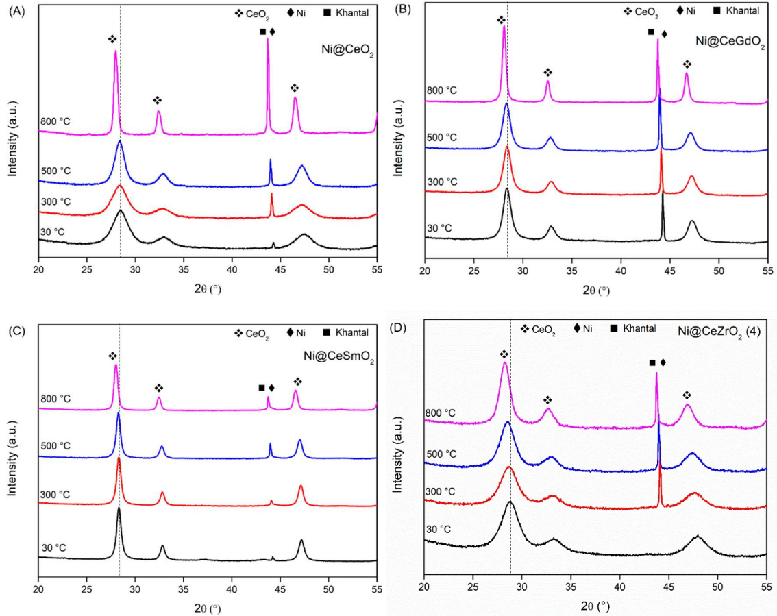
Figure 5.2. Effect of metal dopant by in-situ XRD obtained during reduction process for the (A) Ni@CeO 2 , (B) Ni@CeGdO 2 , (C) Ni@CeSmO 2 and (D) Ni@CeZrO 2 (4) catalysts.
