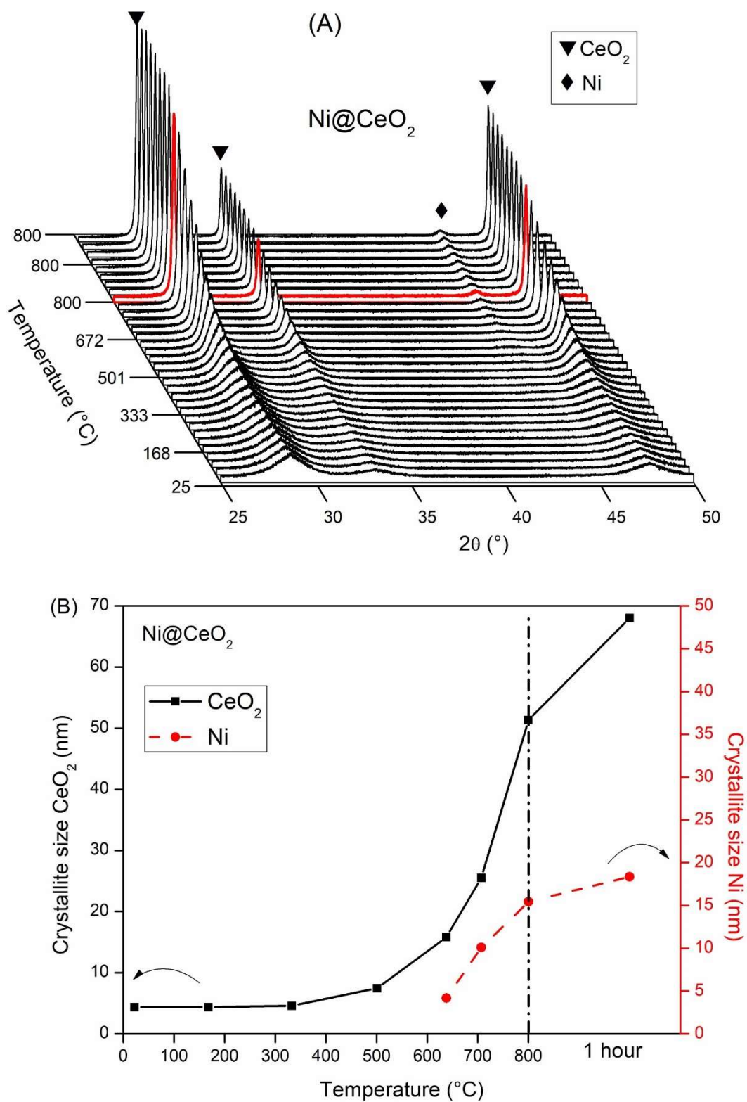
Figure 4.11. (A) X-ray diffraction patterns obtained during reduction from room temperature to 800 °C for Ni@ \text{CeO}_2 ; (B) Crystallite size of \text{Ni}^0 and \text{CeO}_2 during the reduction process.
