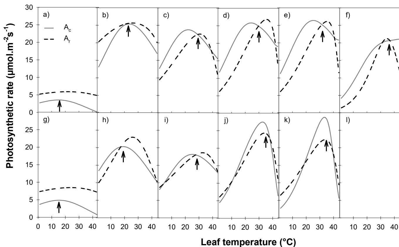
Figure 34—Predicted responses to leaf temperature of the RuBP carboxylation limited (full line, A_c ) and the RuBP regeneration limited (dotted line, A_r ) assimilation rates at 400 ppm \text{CO}_2 and growth temperatures of 5°C (a-g), 10°C (b-h), 20°C (c-i), 25°C (d-j), 30°C (e-k) and 35°C (f-l). Data are for two alfalfa genotypes of temperate (a-l, G3) and Mediterranean (g-l, 7_7) origins. Arrows indicate the predicted thermal optimum.
