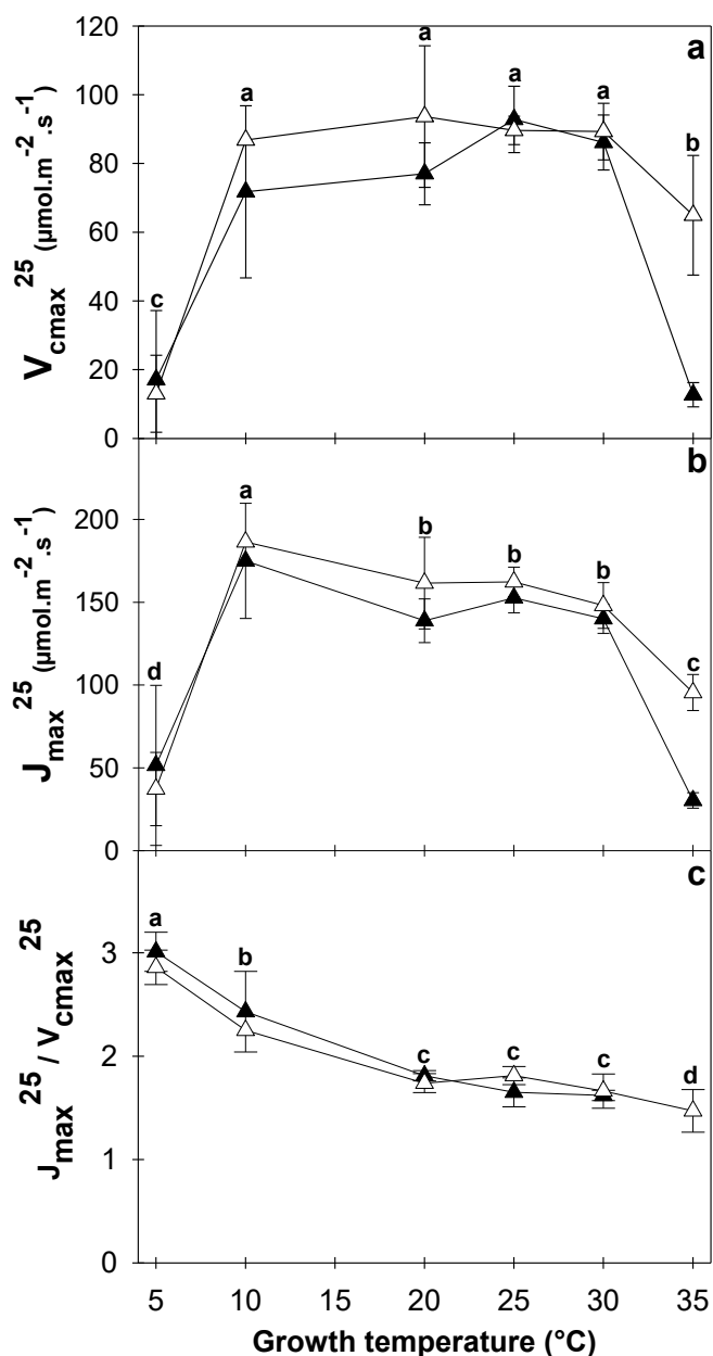
Figure 32—Impact of growth temperature on the maximum catalytic rate of Rubisco ( V_{cmax}^{25} , a), the maximum electron transport rate ( J_{max}^{25} , b) and their ratio (c, J_{max}^{25}/V_{cmax}^{25} ) for two alfalfa genotypes of Mediterranean (filled triangles, 7_7) and temperate (open triangles, G3) origins. The letters indicate homogeneous groups of means between the different growth temperatures (Fisher's LSD test).
