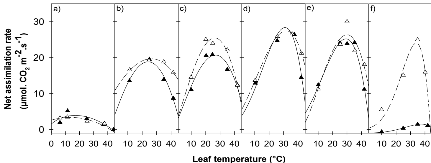
Figure 31—Temperature responses of the net assimilation rate at ambient CO 2 ( A_{400} ) for growth temperatures of 5°C (a), 10°C (b), 20°C (c), 25°C (d), 30°C (e) and 35°C (f). Data are presented for two alfalfa cuttings of Mediterranean (filled triangles, 7_7 cutting) and temperate (open triangles, G3 cutting) origins. Lines represent fits of Eqn 6. Each point is the average of measurements on three to four mature leaves (node ranks 12-16).
