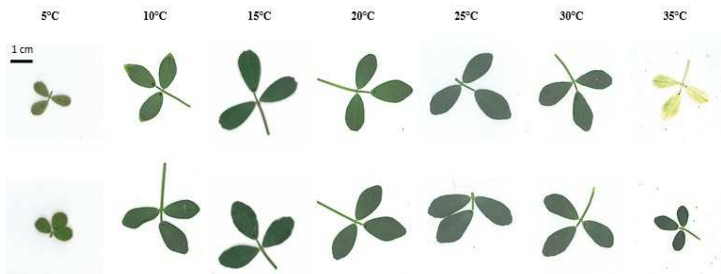
Figure 29—Alfalfa leaves of Mediterranean (Barmed cv) and temperate (Harpe cv) cultivars grown at different temperatures. Measurements were performed on the youngest mature leaf of the main stem at the end of the experiment (i.e. node ranks 8-9). The horizontal bar represents 1 cm.
