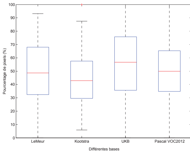
(a) Harris
