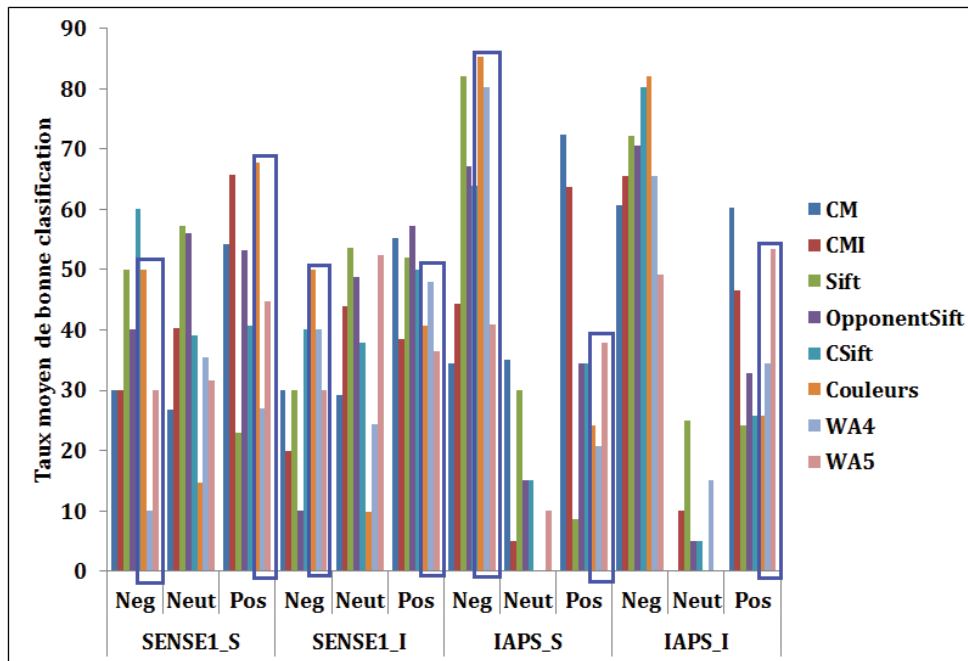
(a) Signature visuelle BOW
